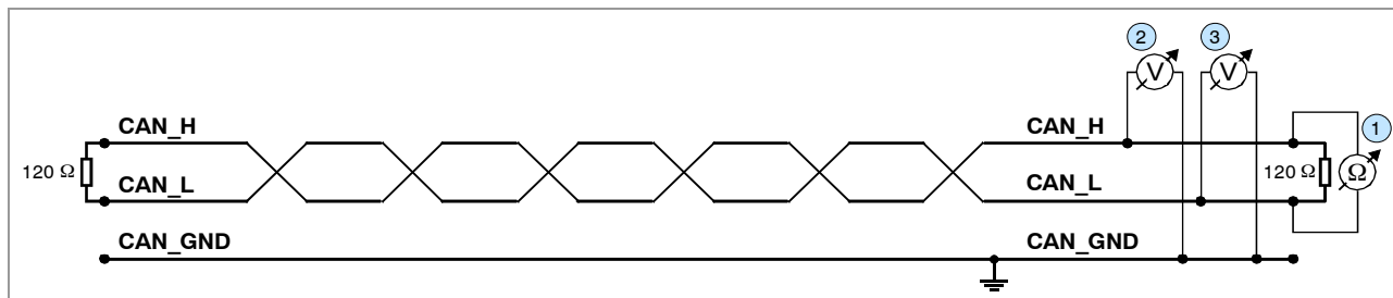
Figure 13: Simplified diagram of a CAN network
