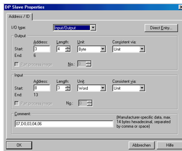
Fig. 5.2.5: Configuration example
