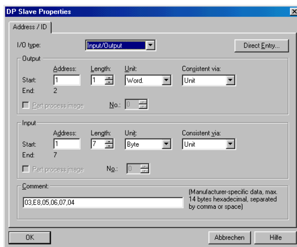
Fig. 5.2.4: Configuration example
