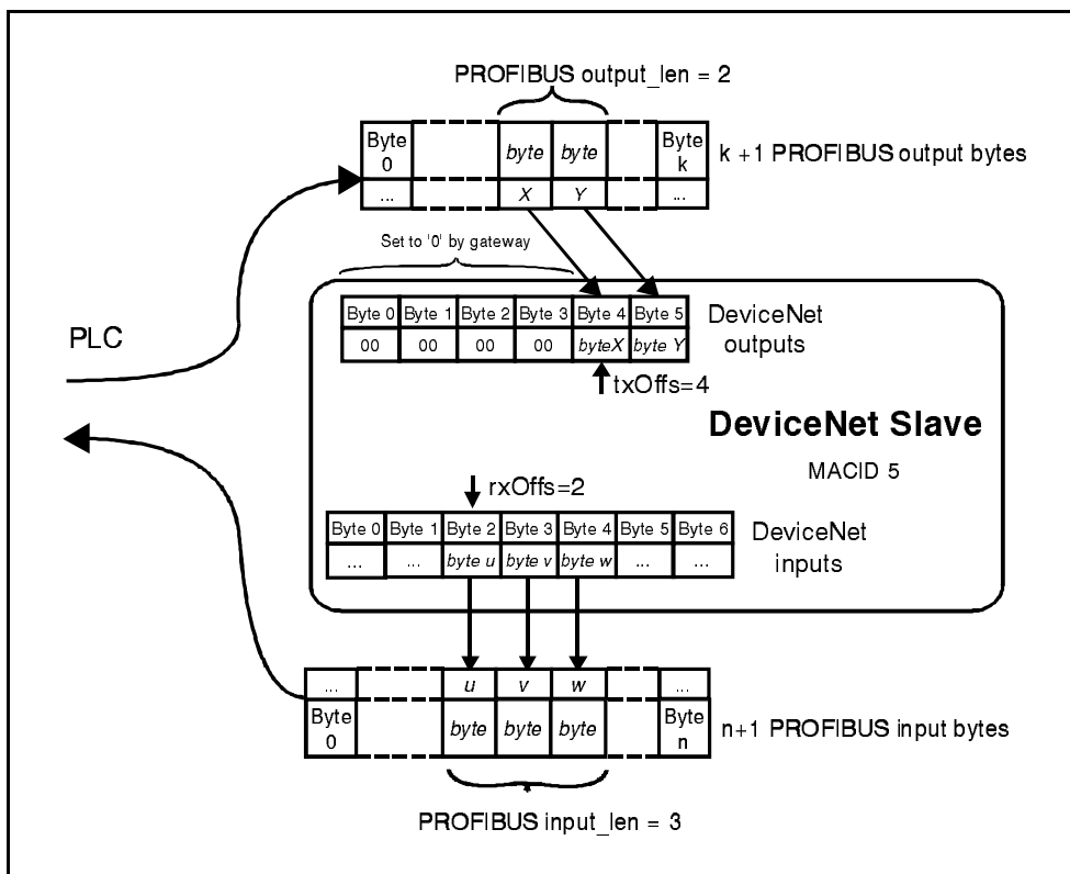
Fig. 5.5.2: Configuration example
