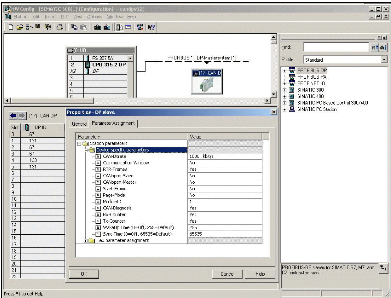
Fig. 5.1.2: Setting the parameters in the DP-slave properties window
