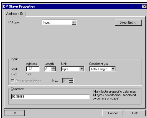
Fig. 5.1.4: Example: Configuration of input data
