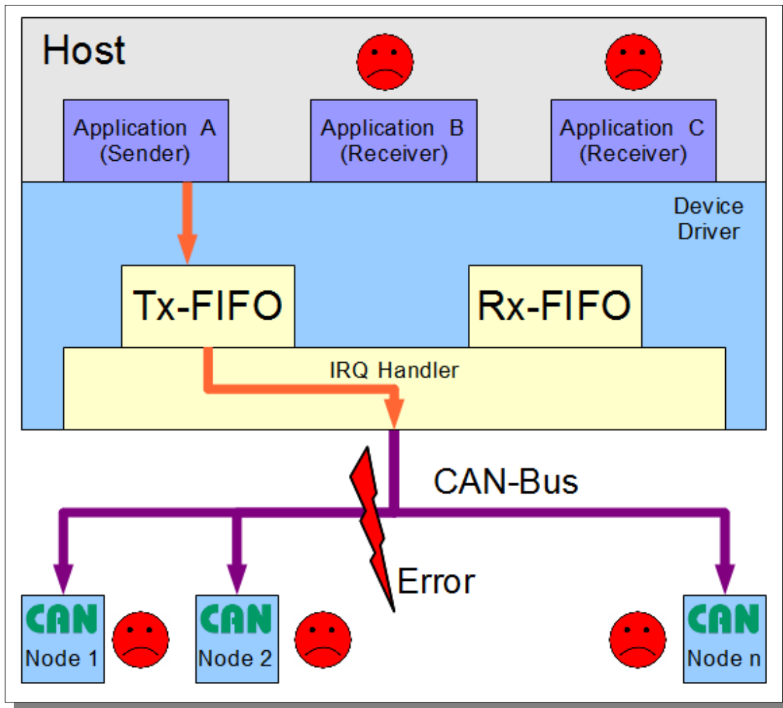
Figure 9: Interaction without IPC
