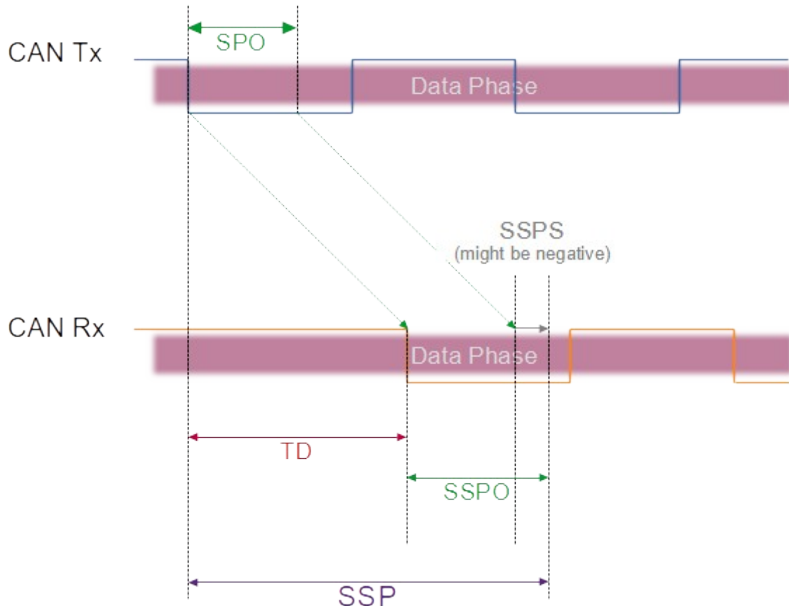
Figure 17: SSP configuration in NTCAN TDC Automatic Mode.
