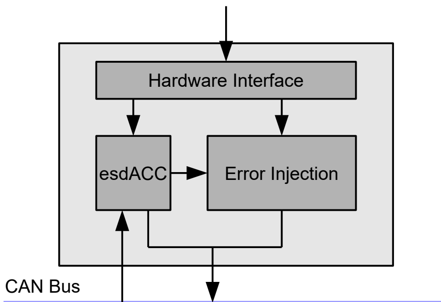
Figure 13: Overview of esdACC Error Injection
