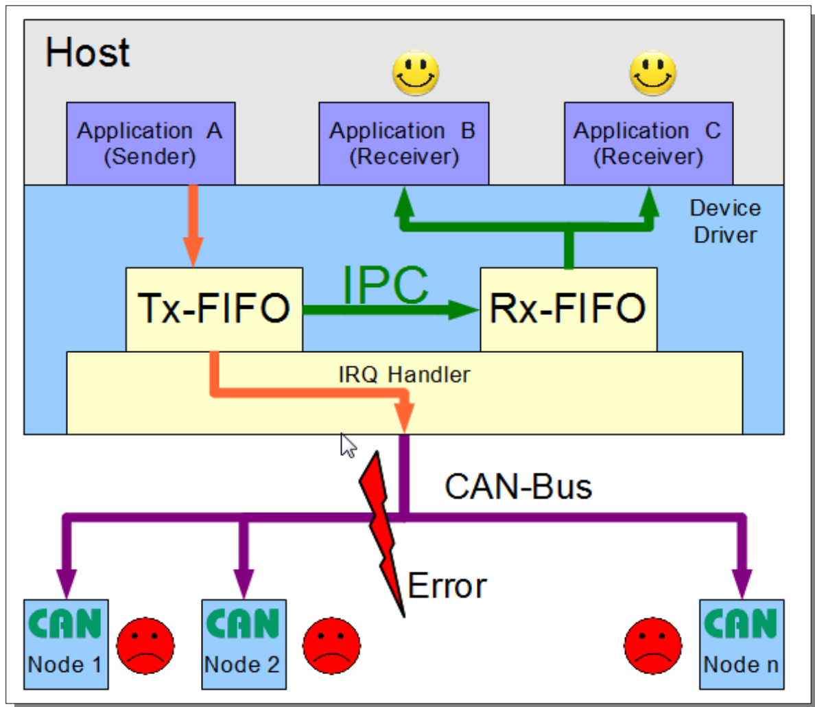
Figure 8: Interaction with IPC
