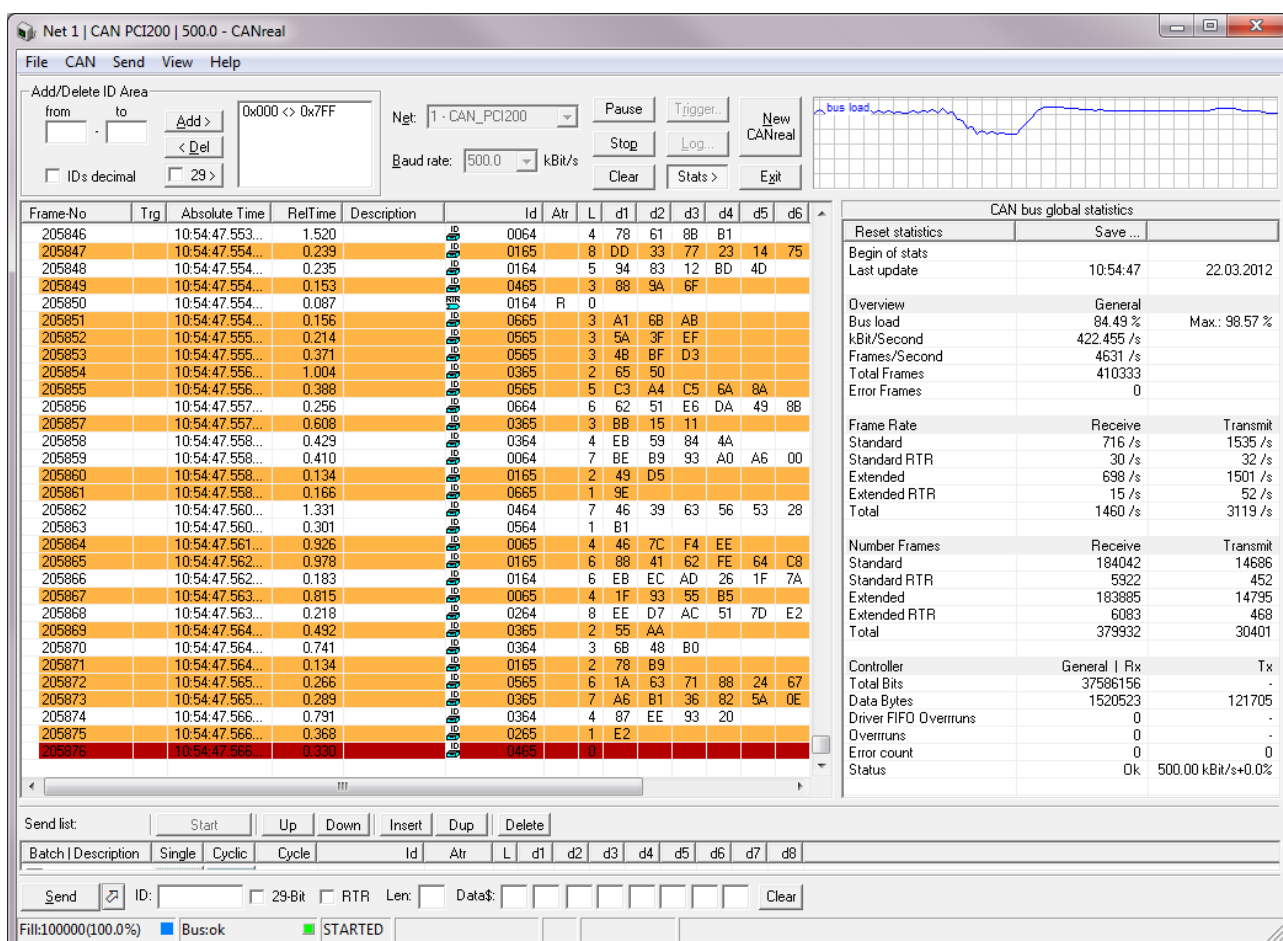
Figure 19: CANreal Bus Monitor
