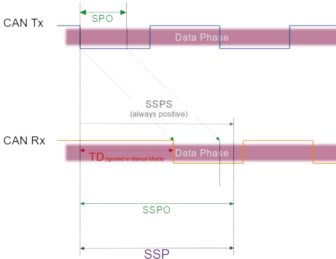
Figure 18: SSP configuration in NTCAN TDC Manual Mode.
